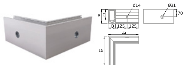
SV-1702-C OUTSIDE
