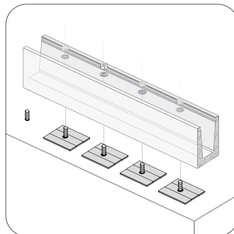
Drainage profile
