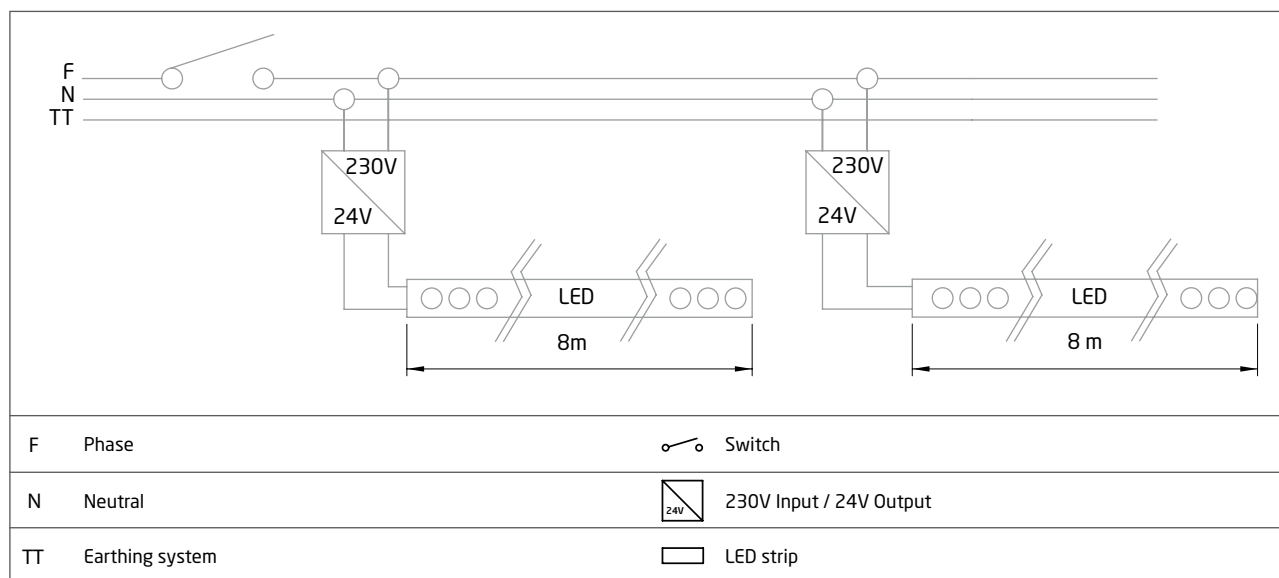
Wiring diagram
